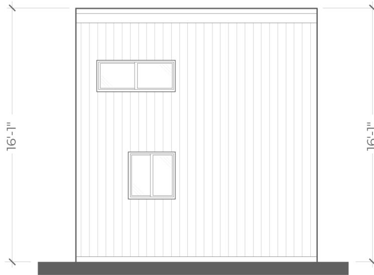
ELEVATION D
