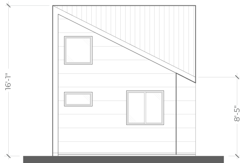
ELEVATION C
