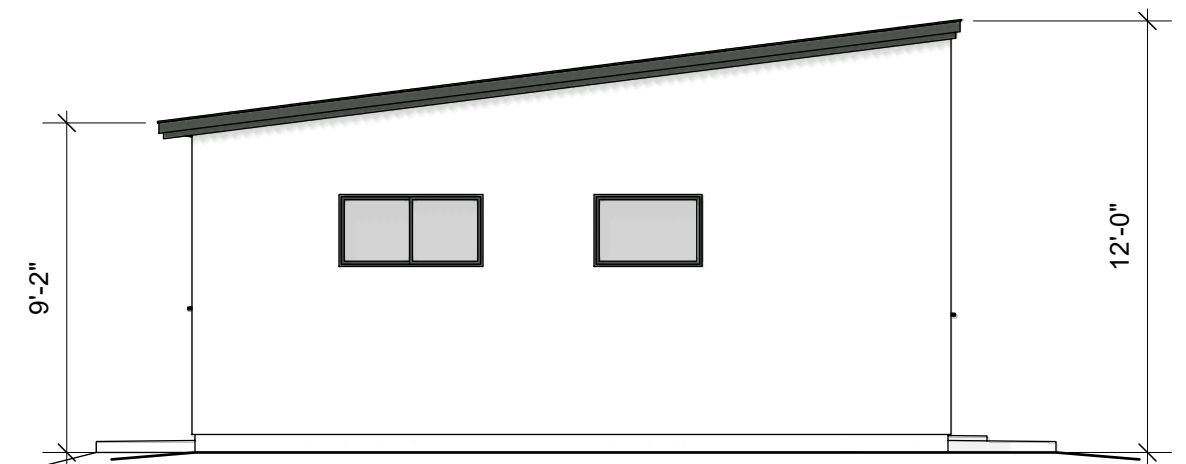
ELEVATION D
