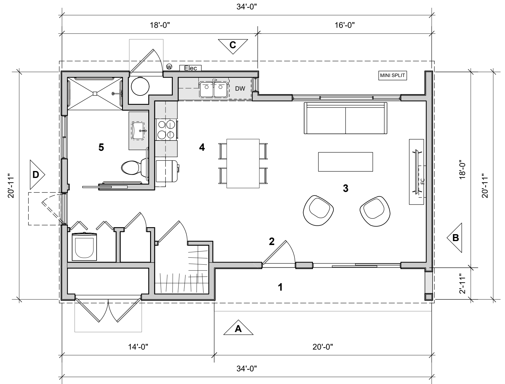
FLOOR PLAN
