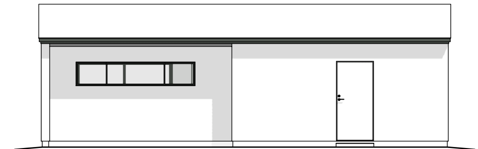
ELEVATION C
