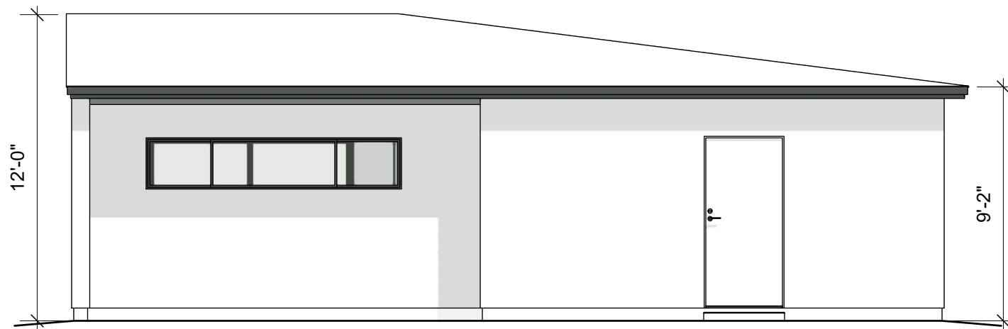
ELEVATION C
