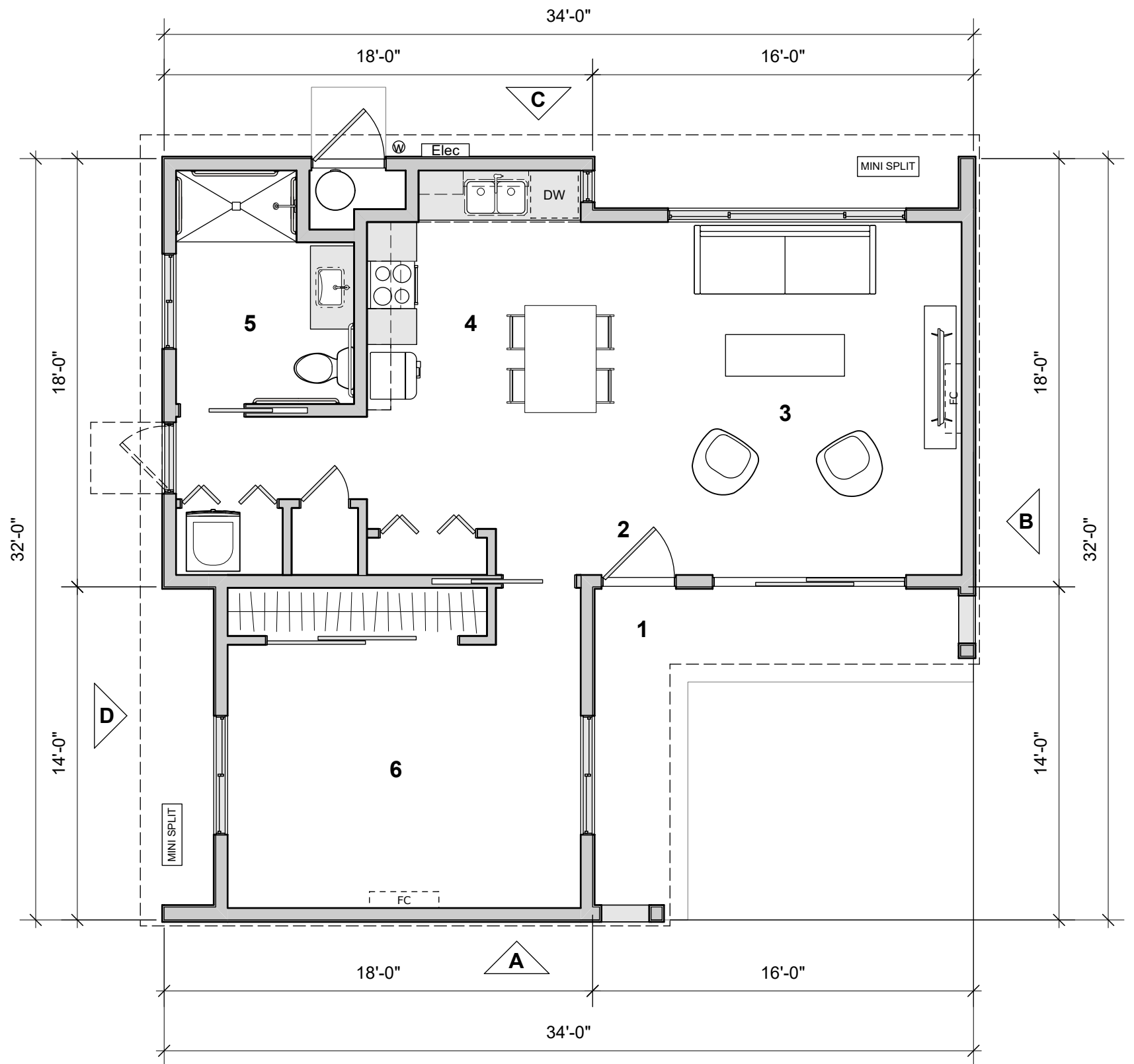
FLOOR PLAN
